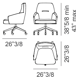
Low backrest
