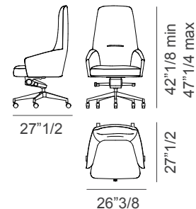
High backrest
