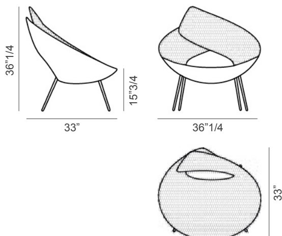
Lock Ego lounge chair
