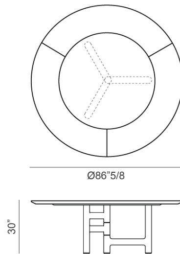
Option C Ø86"5/8 x 30"H
