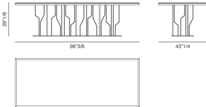
Ginza Fixed Table 1: 98 3/8" W x 43 1/4" D x 29 1/8" H
