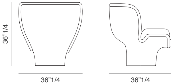
Elda Lounge Chair: 36"1/4W x 36"1/4D x 36"1/4H
