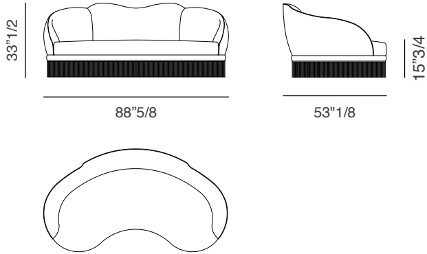
Daisy Sofa: 88"5/8W x 53"1/8D x 33"1/2H
