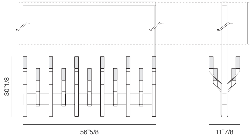
Narita Suspension Lamp: 56"5/8W x 11"7/8D x 30"1/8H
