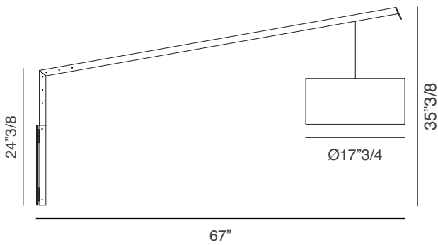
Angelica Wall Lamp 2: 67"W x 17"3/4D x 35"3/8D
