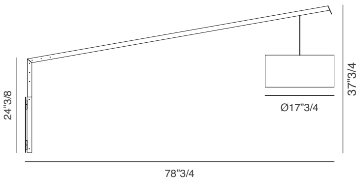
Angelica Wall Lamp 3: 78"3/4W x 17"3/4D x 37"3/4D
