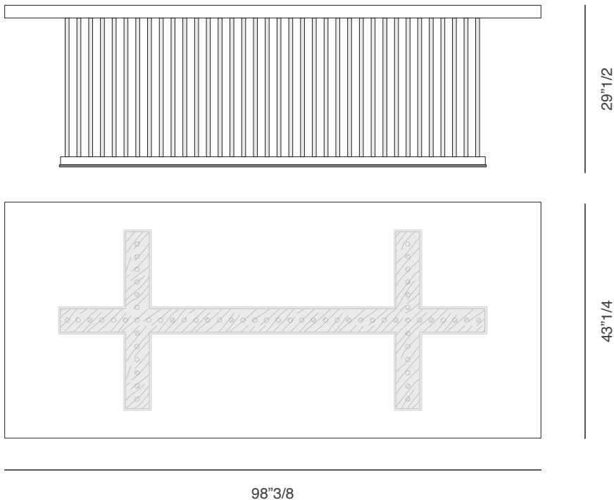
Schubert Fixed Table 1: 98"3/8W x 43"1/4D x 29"1/2H
