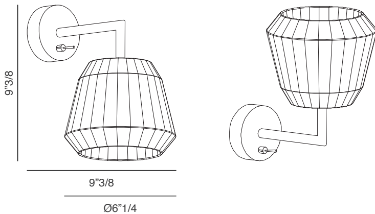
Loto Wall Lamp (with Switch): Ø6"1/4 x 9"3/8D x 9"3/8H
