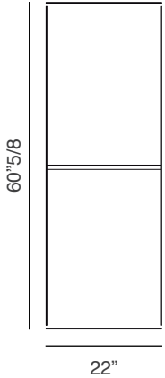
Blade High Cabinet Frame 0M1452CC: 22"W x 19"5/8D x 60"5/8H Frame for 1 unit high cabinet in melamine linen finish. Top covered in saddle leather.
