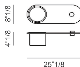
Cup Holder: 25"1/8W x 8"1/8D x 4"1/8H
