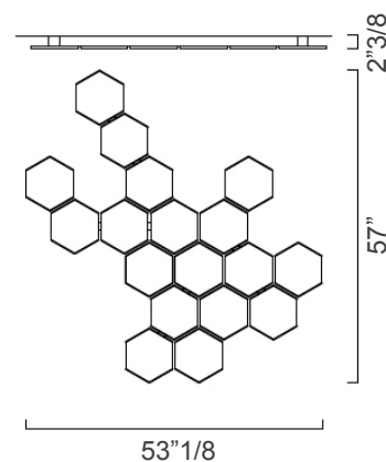
(F) 7372/A
