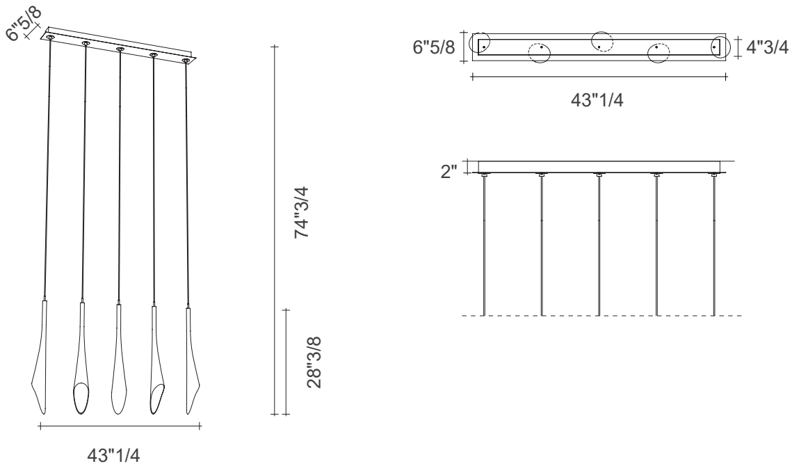
Linear five light pendant
