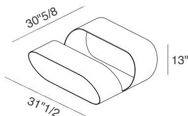
Base Only
