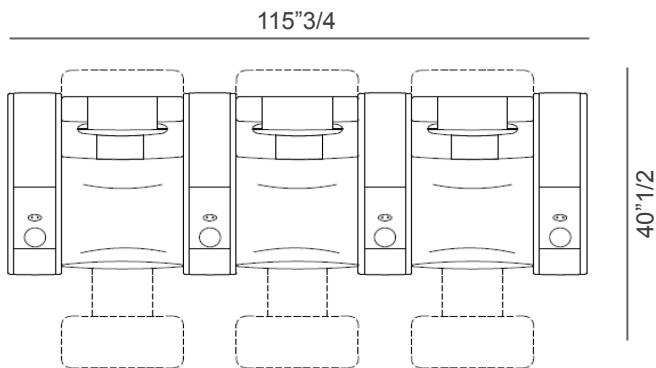
Composition D 3 seats, straight
