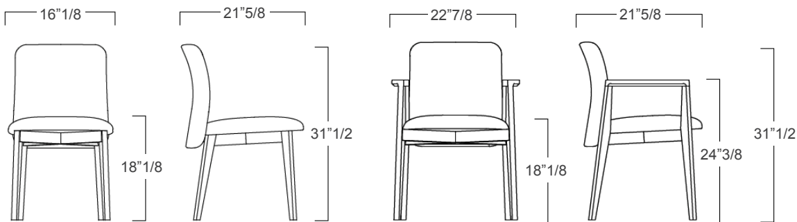
A) Without armrests - Cod. FG53410
