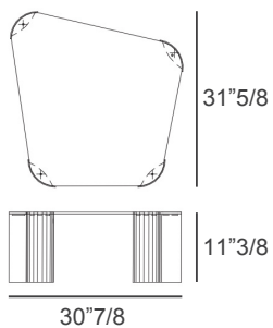
Trapezoidal - D)
