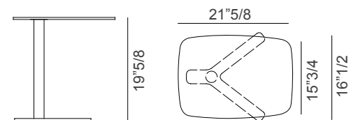
Size D - Rectangular top with rounded ends
