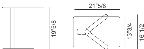
Size C - Rectangular top
