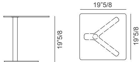
Size B - Square top
