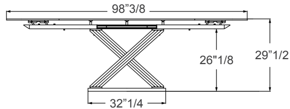
2 Extension Leaves Open
