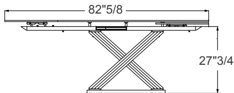
1 Extension Leaf Open
