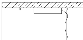
Hook with canopy, metal cables and ceiling cable gripper (F)
