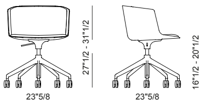
5-spoke Pyramidal Base (Adjustable Height)
