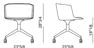
4-spoke Pyramidal Base (Fixed Height)
