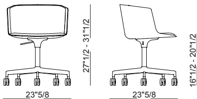
5-spoke Low Base (Fixed or Adjustable Height)
