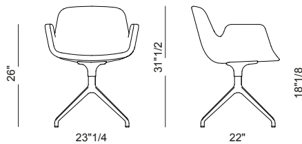
4-spoke Pyramidal Base
