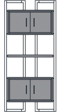
1 shelf & 2 containers (G) Cod. BITO3G
