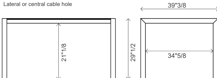
Lateral or central cable hole
